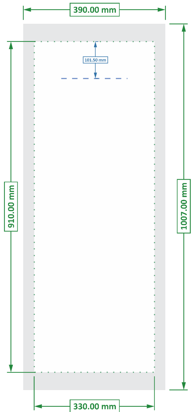
Figure KID-1: Kids Deckchair print dimensions. Bleed marked in grey.
